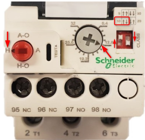
Figure #5 – 036-2 Units Overload Settings
