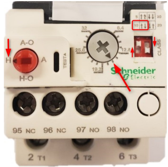
Figure #4 – 036-1 PSC & EON Units Overload Settings
